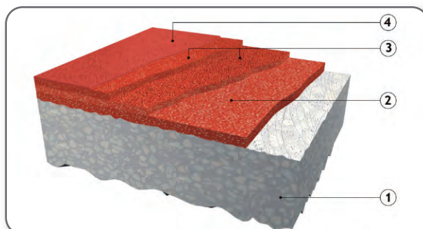
④ Paintex ③ Compotex ② Epoxan ① Soporte
