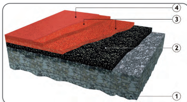
④ Paintex ③ Compotex ② Compotop ① Soporte
